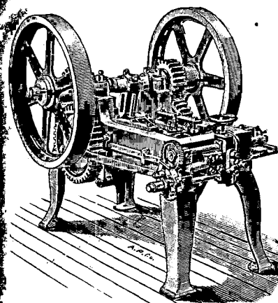
SOLID DIE, DOUBLE STROKE, GEARED RIVET MACHINE.
